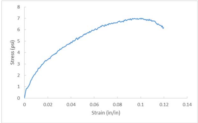
Figure A.114 D8-4, OC= 65.9%, CF= 300 pcf, T=28 days.
