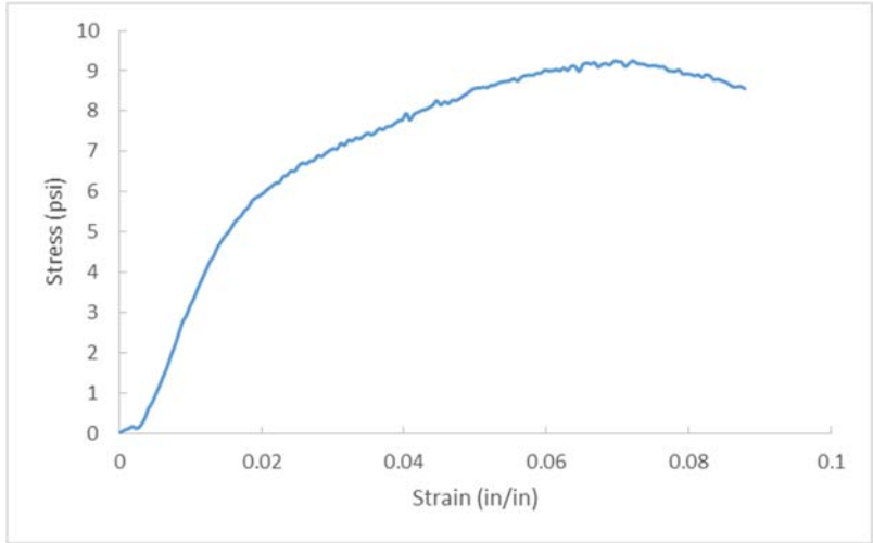
Figure A.324 D57-4, OC= 42.1%, CF= 500 pcf, T=56 days.
