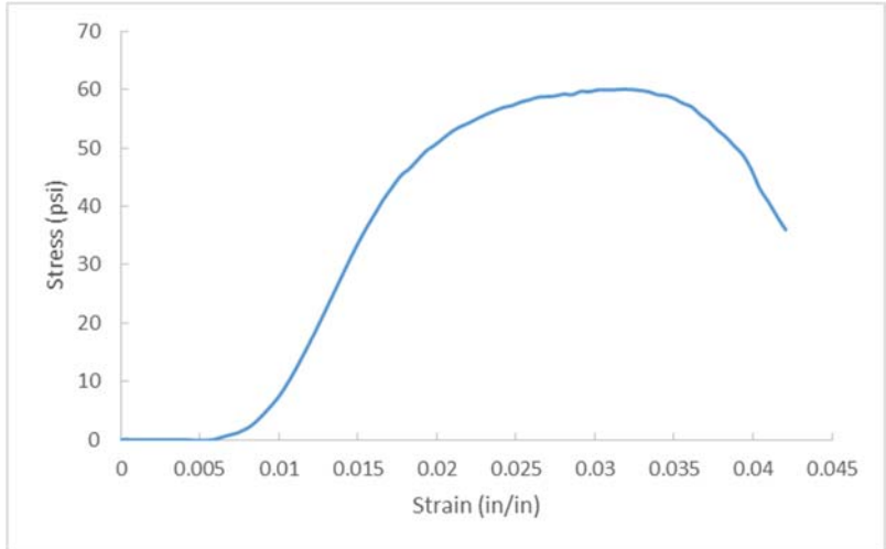
Figure A.282 D34-9, OC= 40.9%, CF= 400 pcf, T=56 days.
