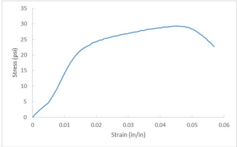
Figure A.132 D15-4, OC= 40.5%, CF= 300 pcf, T=28 days.
