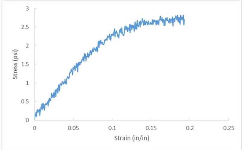
Figure A.120 D10-6, OC= 41.3%, CF= 300 pcf, T=28 days.
