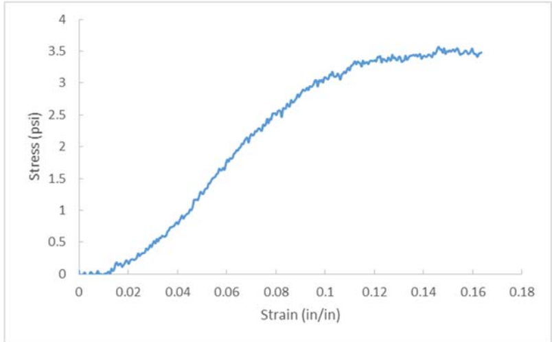
Figure A.228 D10-8, OC= 41.3%, CF= 300 pcf, T=56 days.
