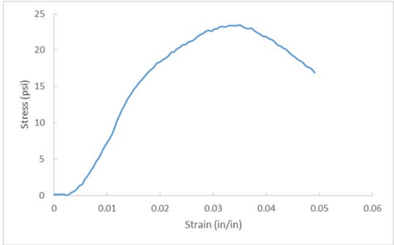
Figure A.150 D26-4, OC= 29.8%, CF= 400 pcf, T=28 days.
