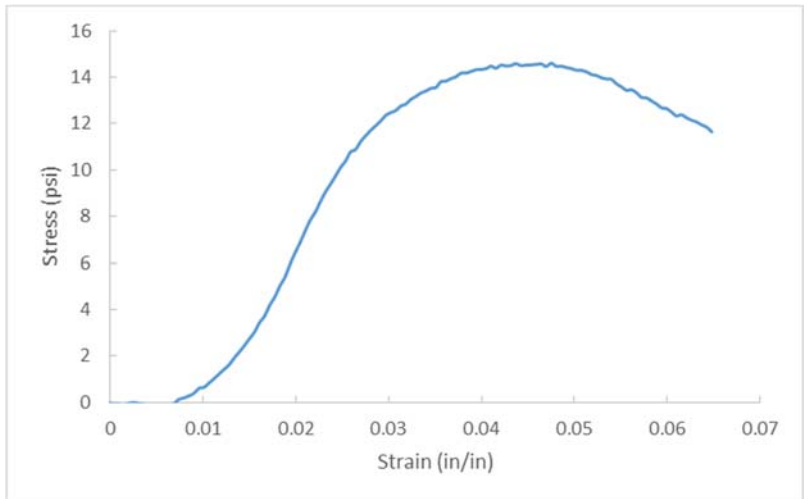
Figure A.209 W51.6, OC= 43.8%, CF= 500 pcf, T=28 days.
