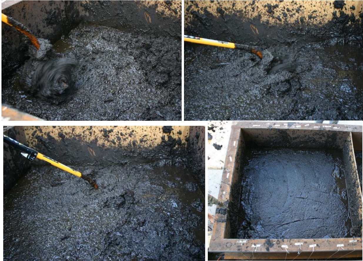
Figure 4.28 Tiller in soil prior to cement introduction.
