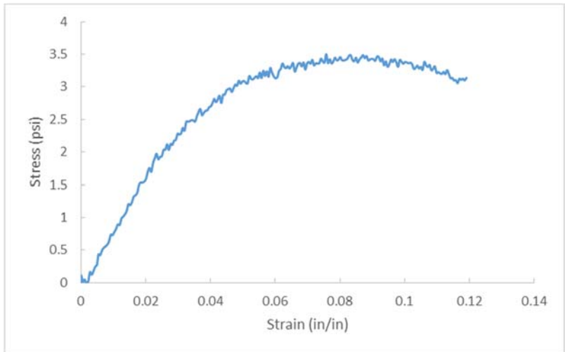
Figure A.203 W49-5, OC= 43.8%, CF= 300 pcf, T=28 days.
