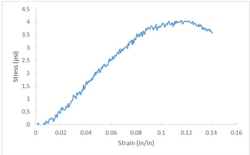
Figure A.121 D11-4, OC= 27.8%, CF= 300 pcf, T=28 days.
