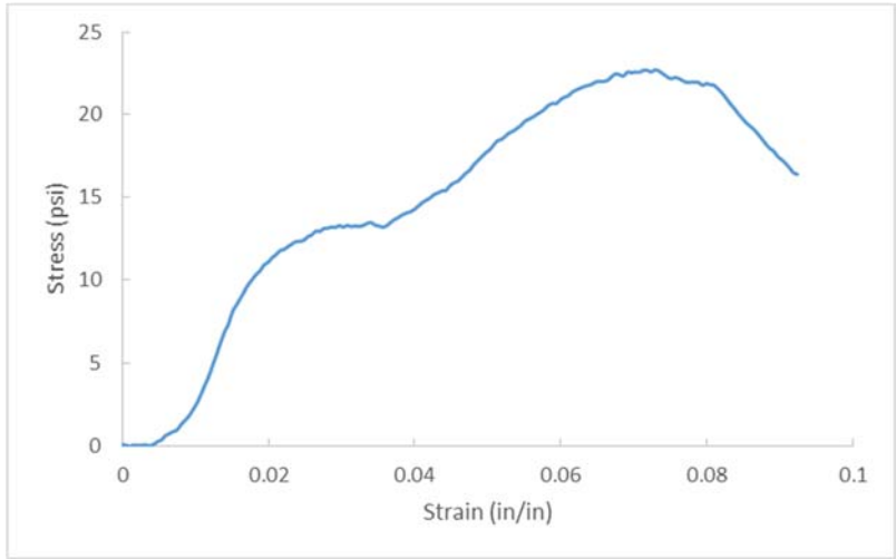
Figure A.140 D17-6, OC= 19.2%, CF= 300 pcf, T=28 days.
