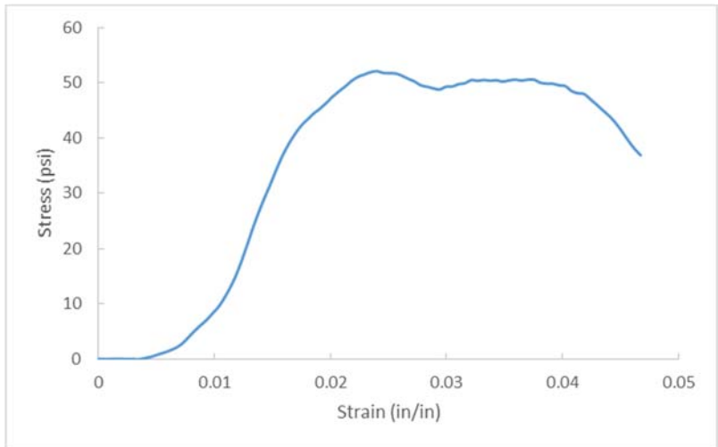
Figure A.251 D19-7, OC= 8.5%, CF= 300 pcf, T=56 days.
