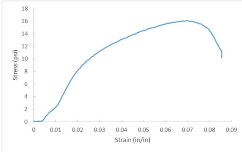
Figure A.180 D37-4, OC= 18.9%, CF= 200 pcf, T=28 days.
