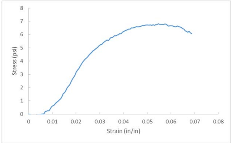
Figure A.318 W50-9, OC= 43.8%, CF= 400 pcf, T=56 days.
