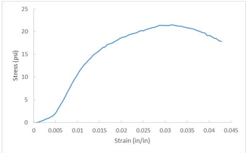
Figure A.151 D26-5, OC= 29.8%, CF= 400 pcf, T=28 days.
