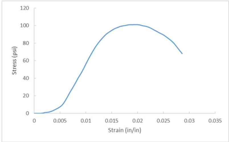
Figure A.273 D31-9, OC= 11.8%, CF= 400 pcf, T=56 days.
