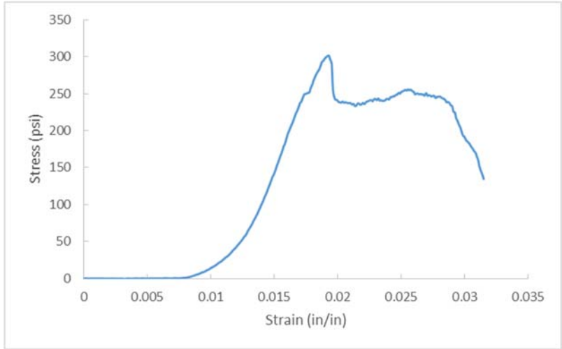
Figure A.201 D48-6, OC= 0.0%, CF= 300 pcf, T=28 days.
