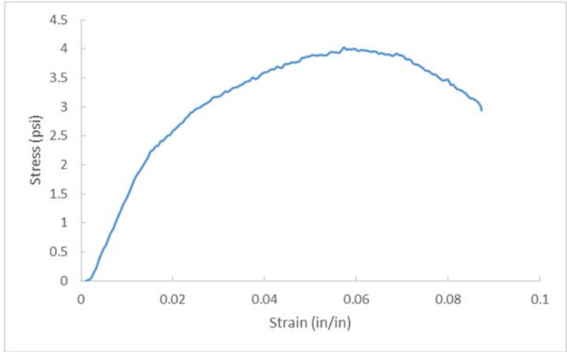
Figure A.111 D4-4, OC= 66.4%, CF= 200 pcf, T=28 days.
