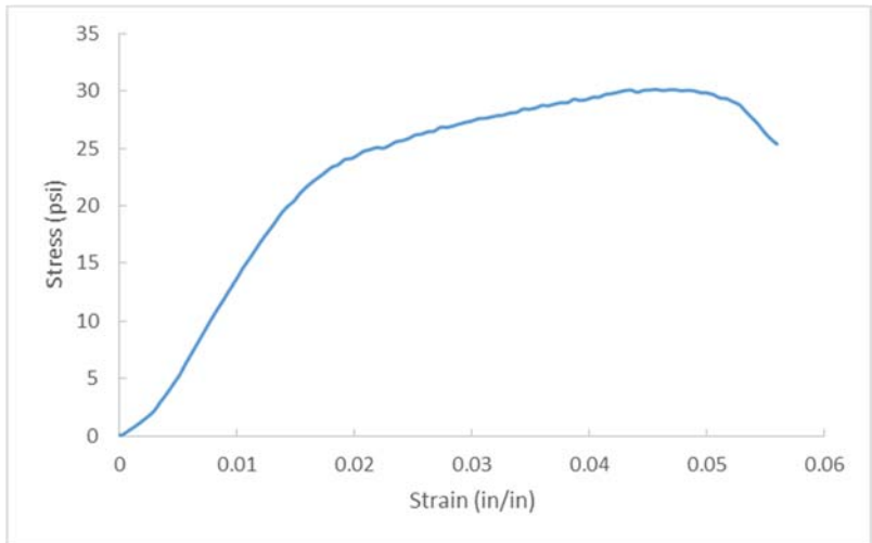
Figure A.134 D15-6, OC= 40.5%, CF= 300 pcf, T=28 days.
