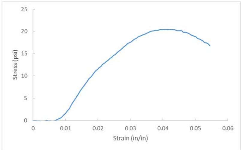
Figure A.152 D26-6, OC= 29.8%, CF= 400 pcf, T=28 days.
