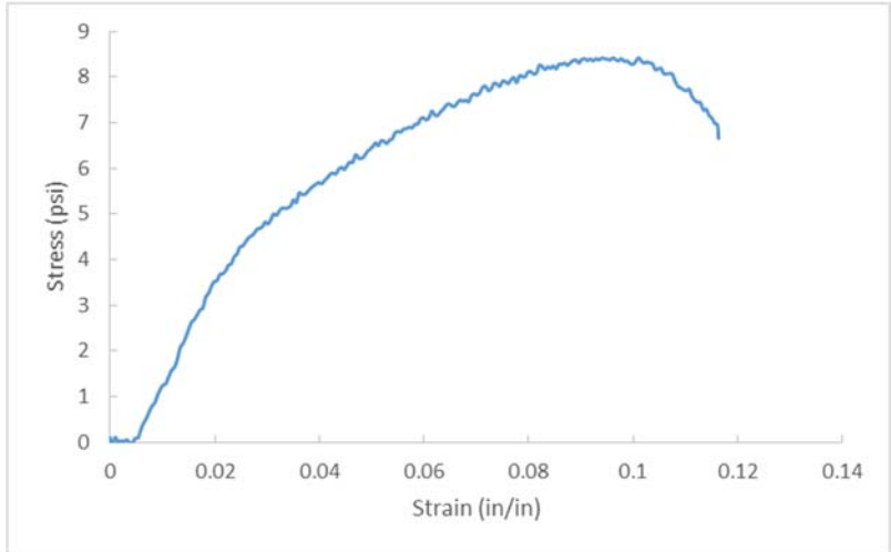
Figure A.213 D57.1, OC= 42.1%, CF= 500 pcf, T=28 days.
