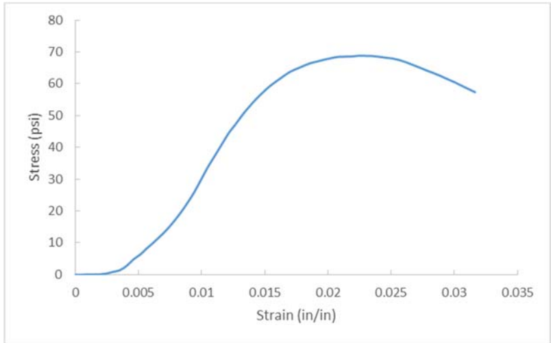
Figure A.274 D32-7, OC= 17.2%, CF= 400 pcf, T=56 days.
