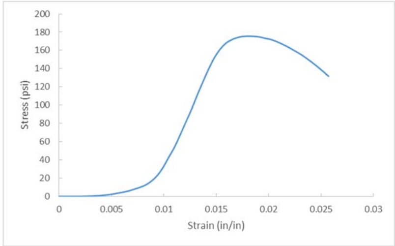
Figure A.270 D30-9, OC= 4.9%, CF= 400 pcf, T=56 days.
