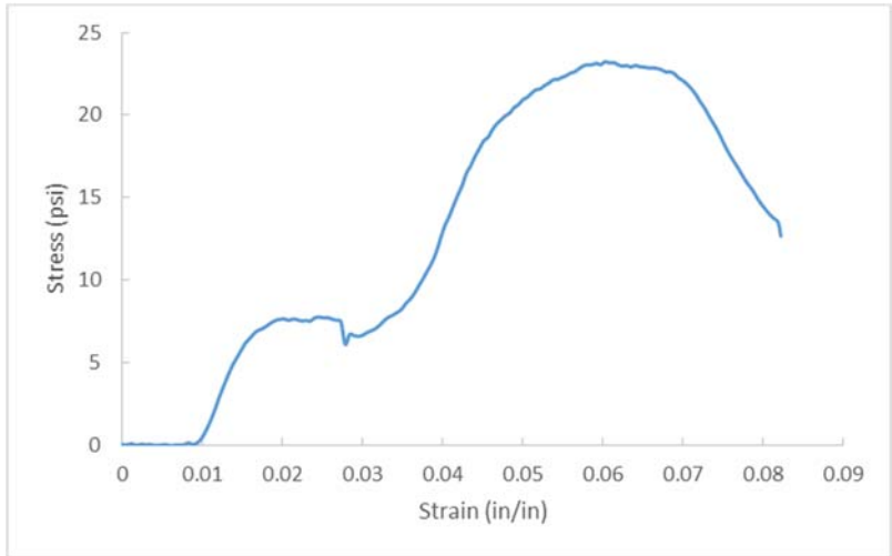
Figure A.139 D17-5, OC= 19.2%, CF= 300 pcf, T=28 days.
