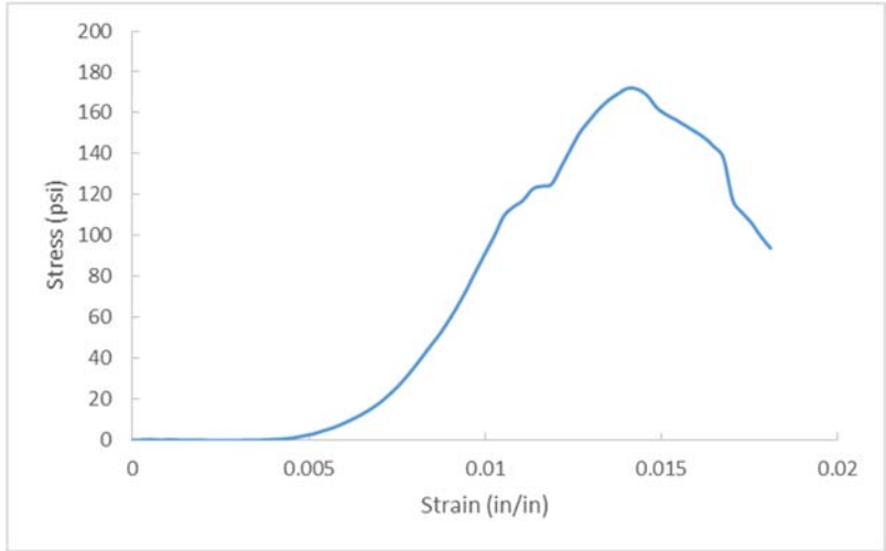
Figure A.306 D46-8, OC= 0.0%, CF= 300 pcf, T=56 days.
