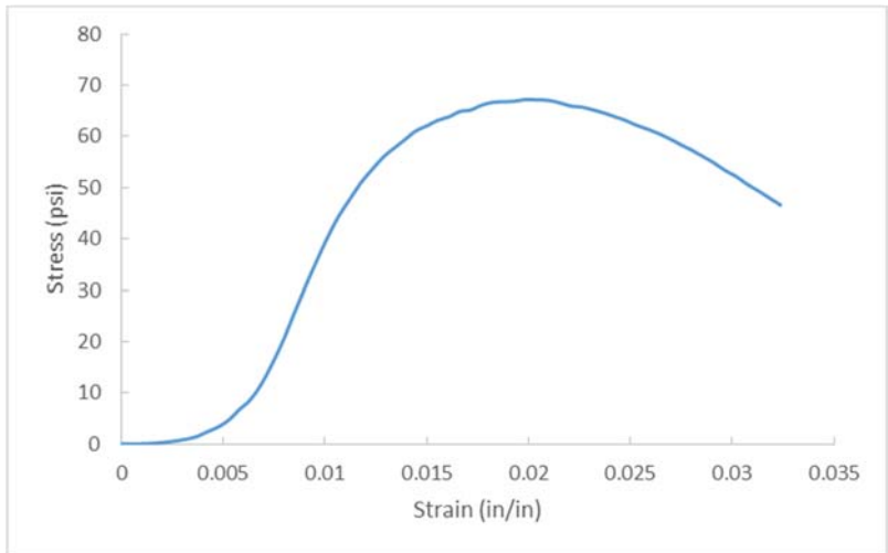
Figure A.275 D32-8, OC= 17.2%, CF= 400 pcf, T=56 days.
