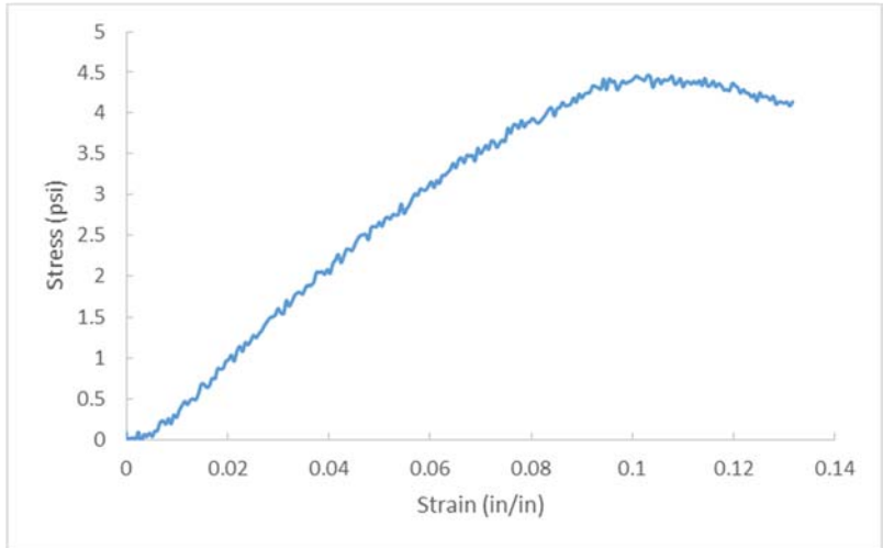
Figure A.122 D11-6, OC= 27.8%, CF= 300 pcf, T=28 days.
