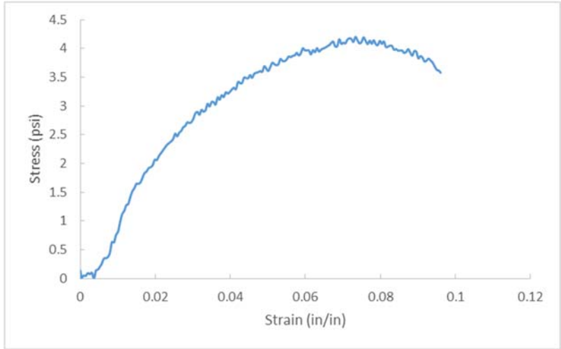
Figure A.297 D43-3, OC= 11.3%, CF= 200 pcf, T=56 days.
