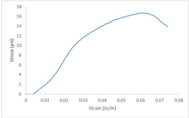
Figure A.291 D38-7, OC= 13.9%, CF= 200 pcf, T=56 days.
