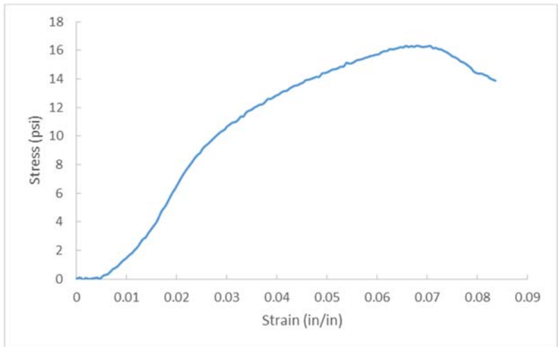
Figure A.289 D37-8, OC= 18.9%, CF= 200 pcf, T=56 days.
