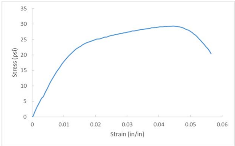
Figure A.133 D15-5, OC= 40.5%, CF= 300 pcf, T=28 days.
