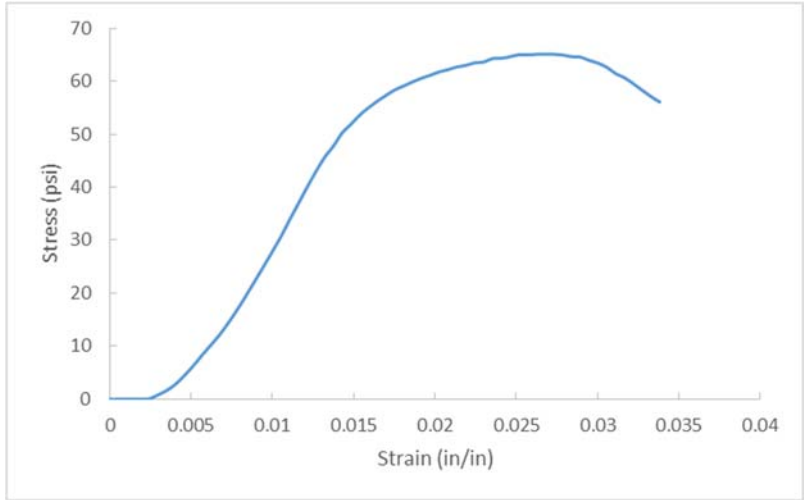
Figure A.168 D32-5, OC= 17.2%, CF= 400 pcf, T=28 days.
