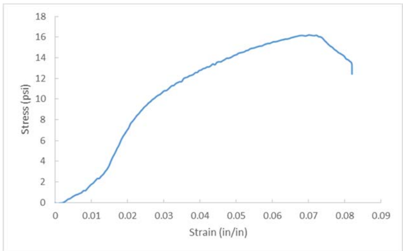
Figure A.290 D37-9, OC= 18.9%, CF= 200 pcf, T=56 days.
