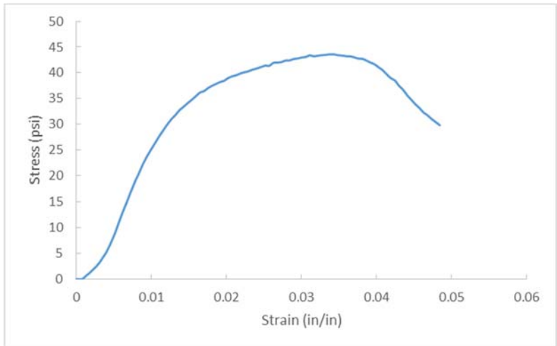
Figure A.212 D55.3, OC= 42.1%, CF= 500 pcf, T=28 days.
