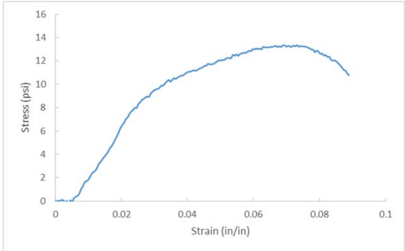
Figure A.285 D36-7, OC= 25.6%, CF= 200 pcf, T=56 days.
