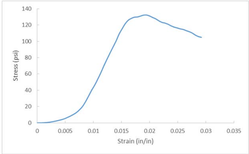
Figure A.129 D14-4, OC= 4.6%, CF= 300 pcf, T=28 days.
