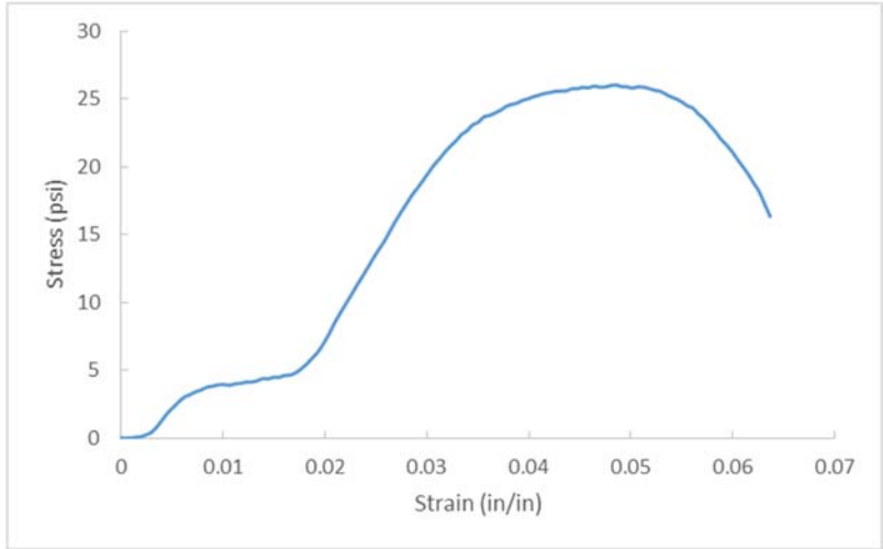
Figure A.138 D17-4, OC= 19.2%, CF= 300 pcf, T=28 days.
